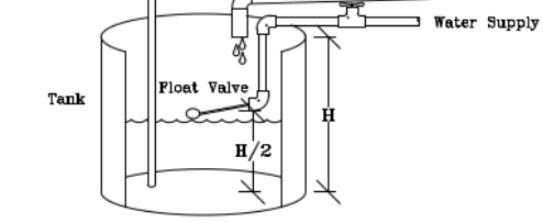
PIPING
